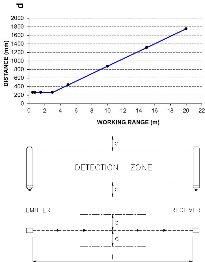
Figure 9 - Minimum distance d
