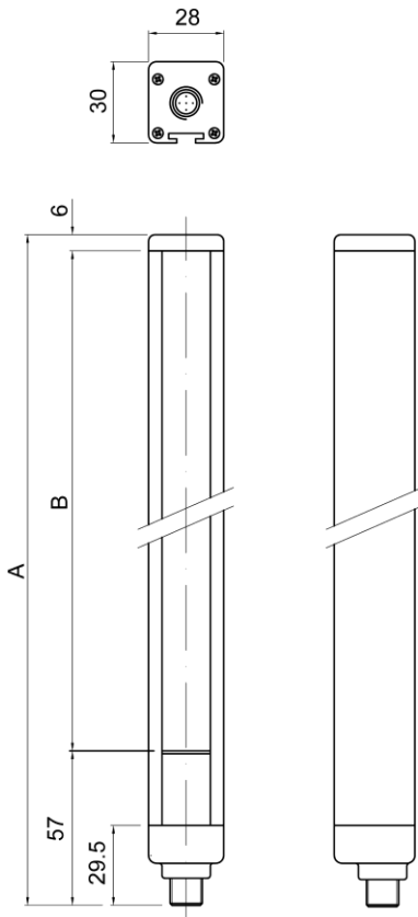
EOS2 A - EOS2 X - EOS2 Slave (Emitter and Receiver)
