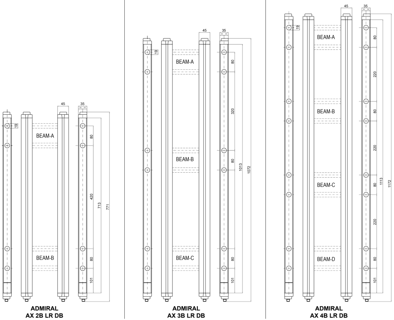
Figure 26 - AX LR DB
