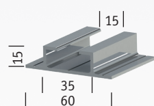
AL 35-15 HB 2009-0030
